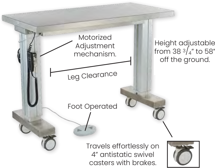
Foot Pedal
