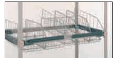
Baskets fit on frames level or at a 10° angle.
