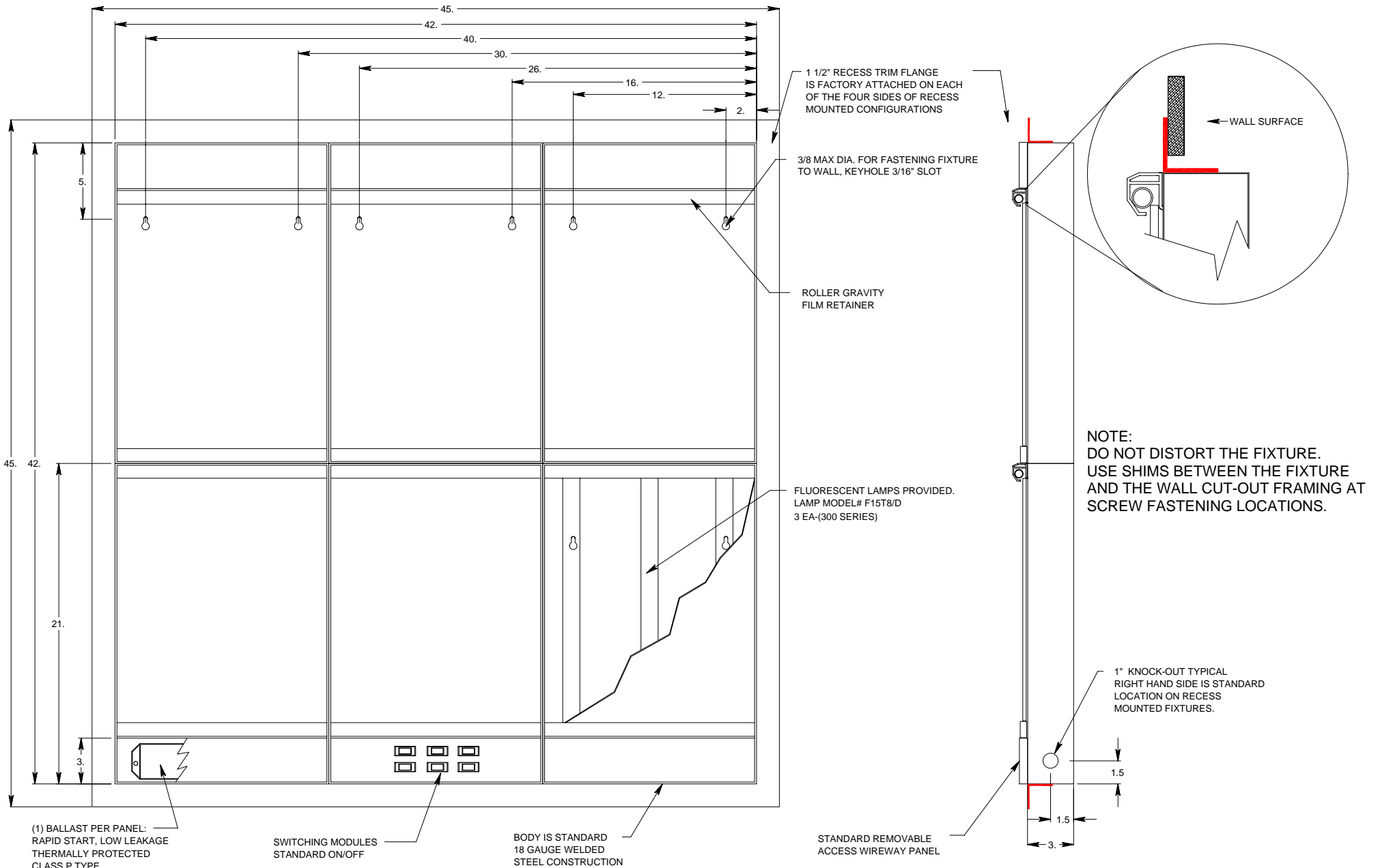
RIGHT VIEW
